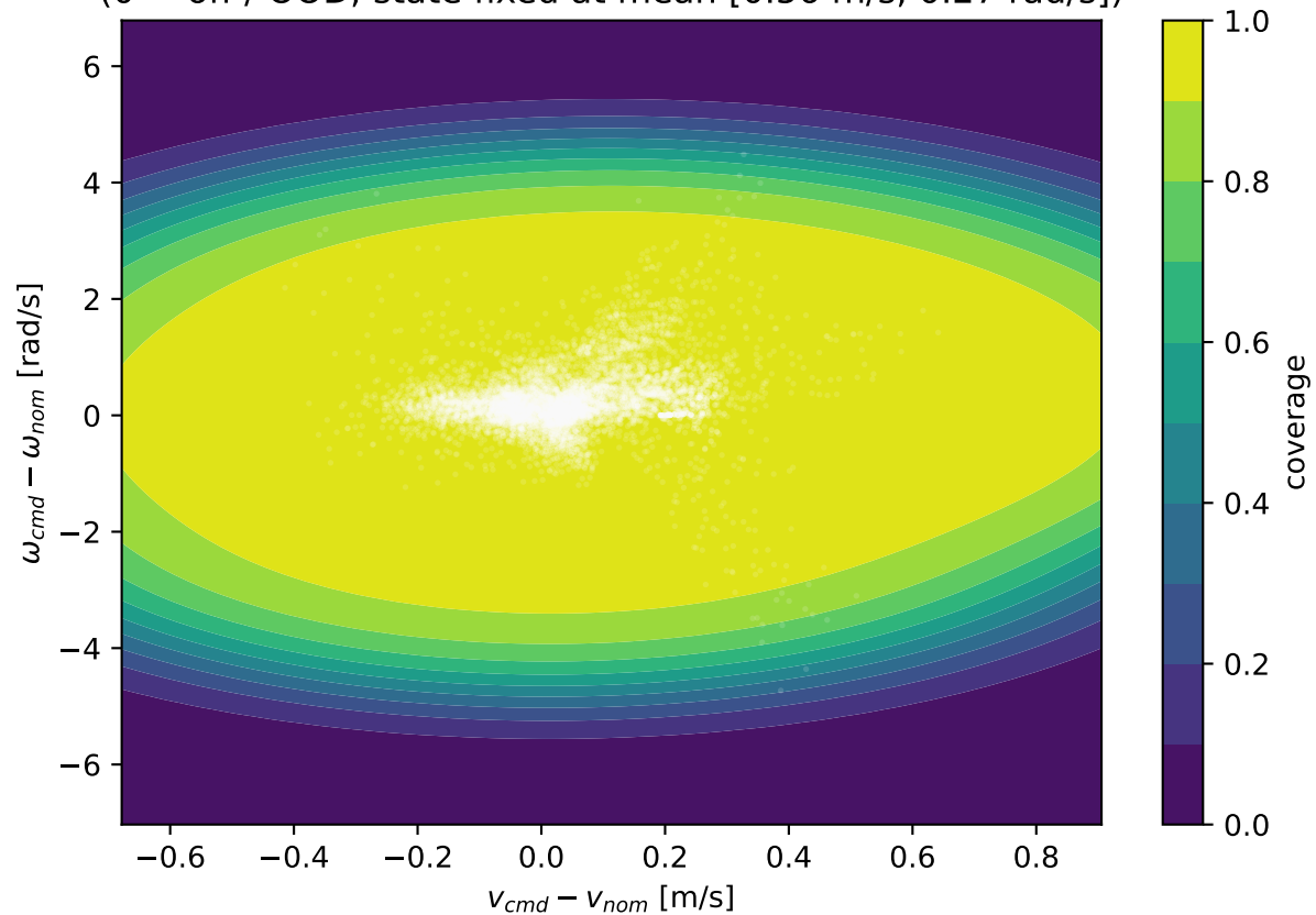
Residual coverage vs command offset (0 = off / OOD; state fixed at mean [0.56 m/s, 0.27 rad/s])
